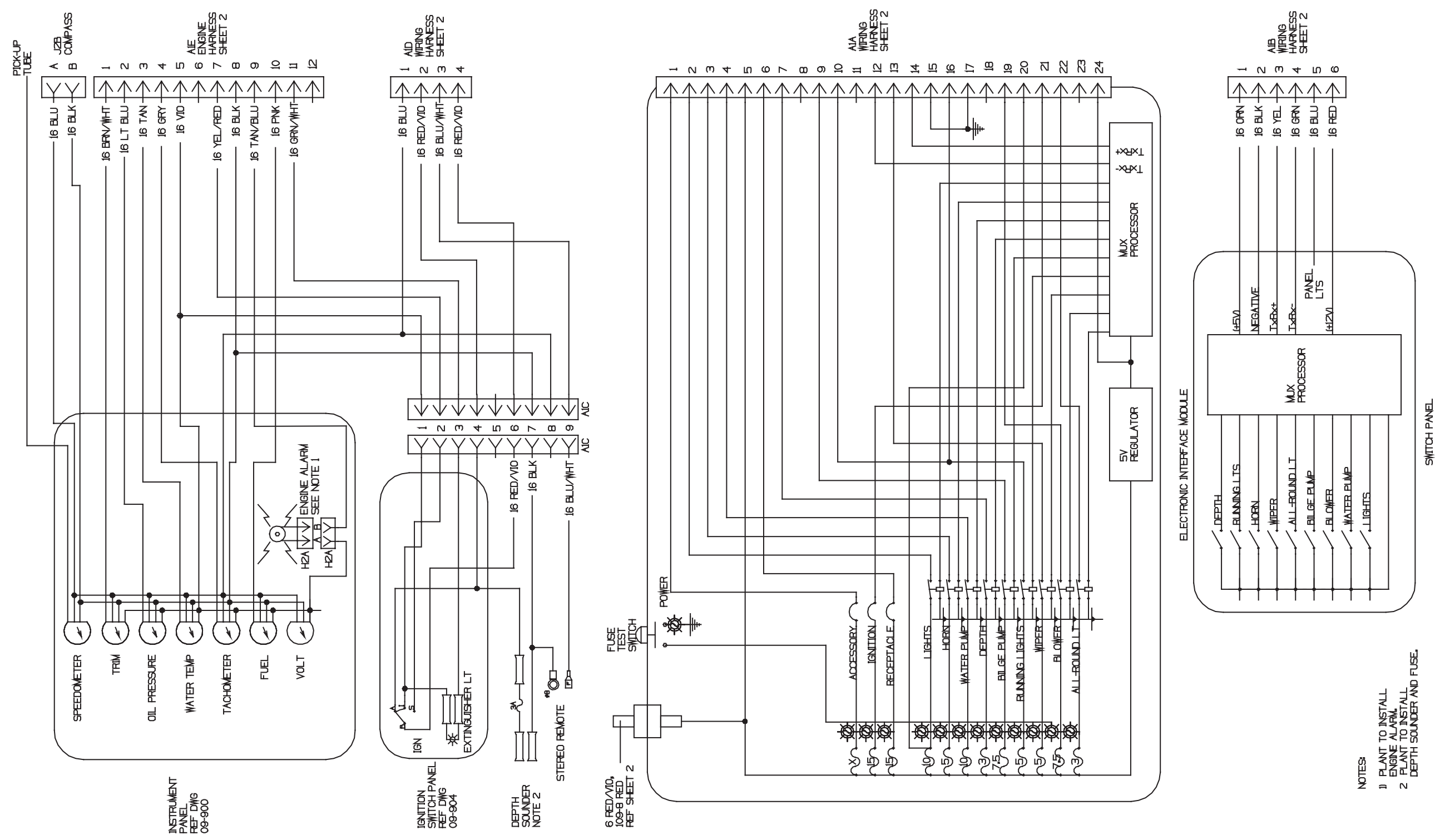
DC WIRING DIAGRAM (FIG. 6.11.1)
