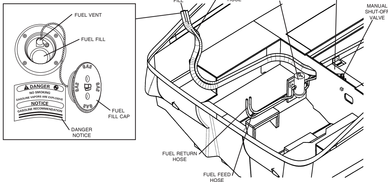
FUEL HOSE ROUTING (DIESEL OPTION) (FIG. 5.2.1)
