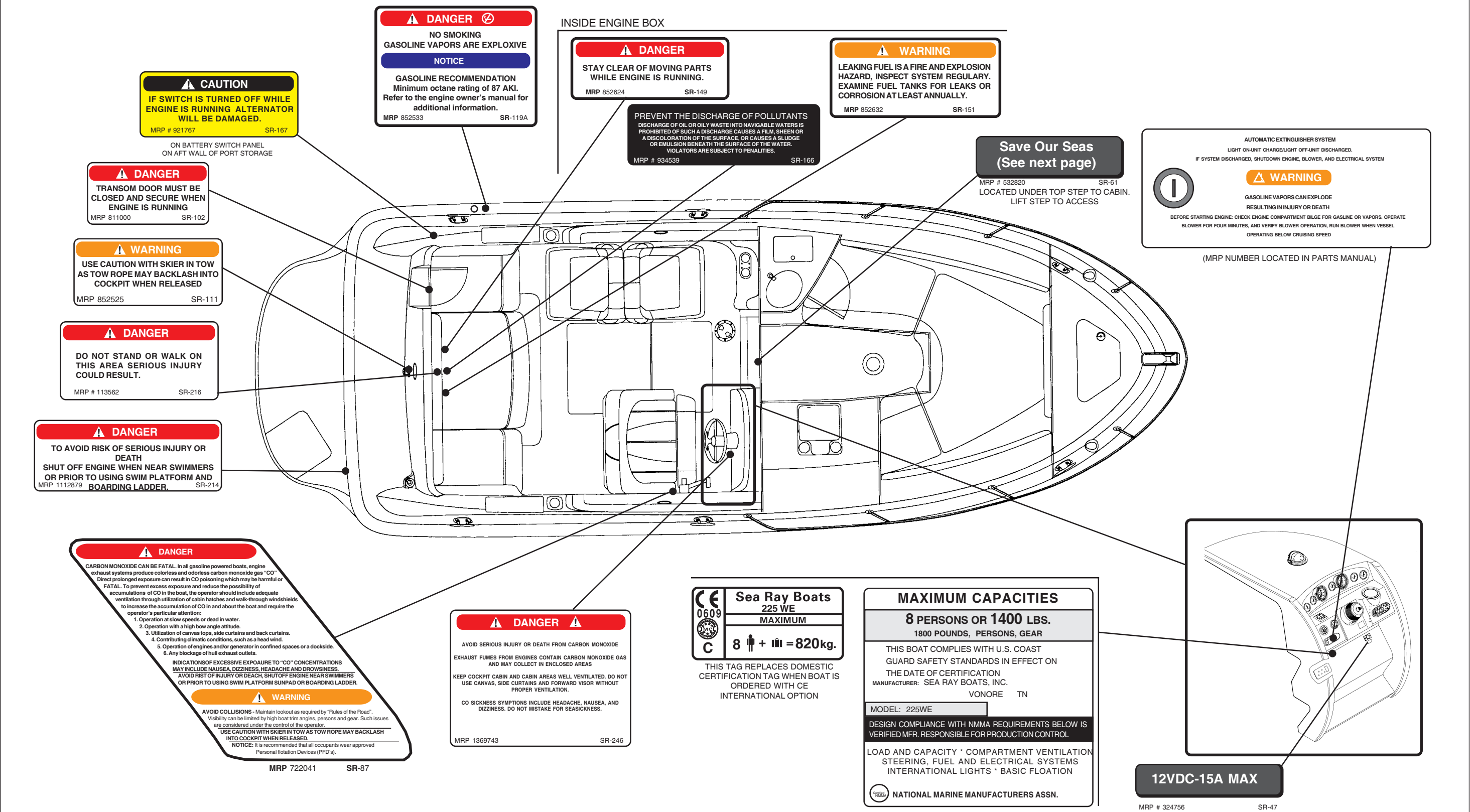
WARNING LABEL LOCATIONS (FIG. 1.17.1)
