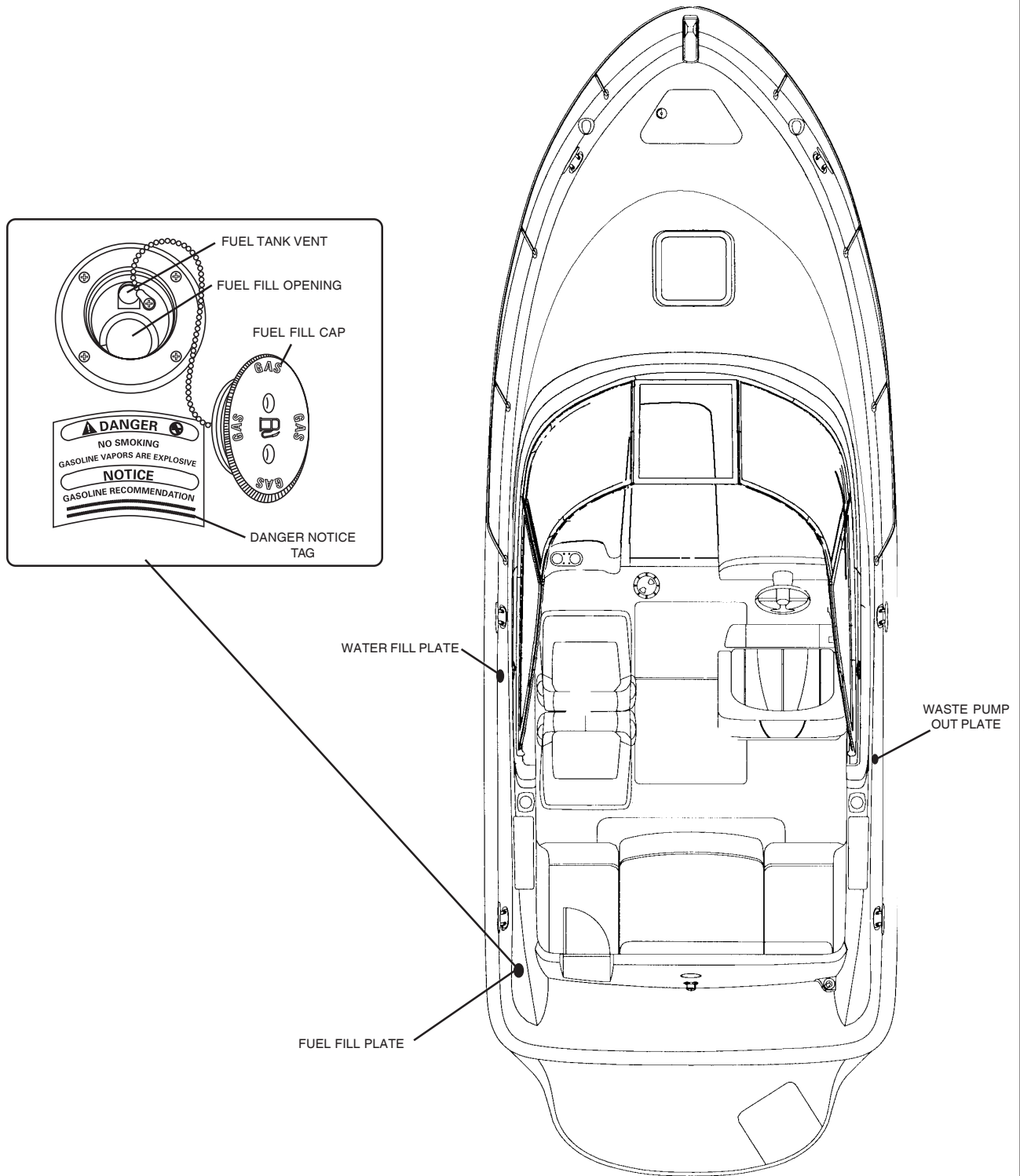
FUEL FILL LOCATION (FIG. 5.5.1)
