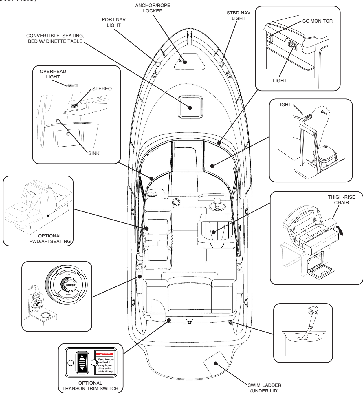
ACCESSORIES AND LOCATION (FIG. 7.1.1)
