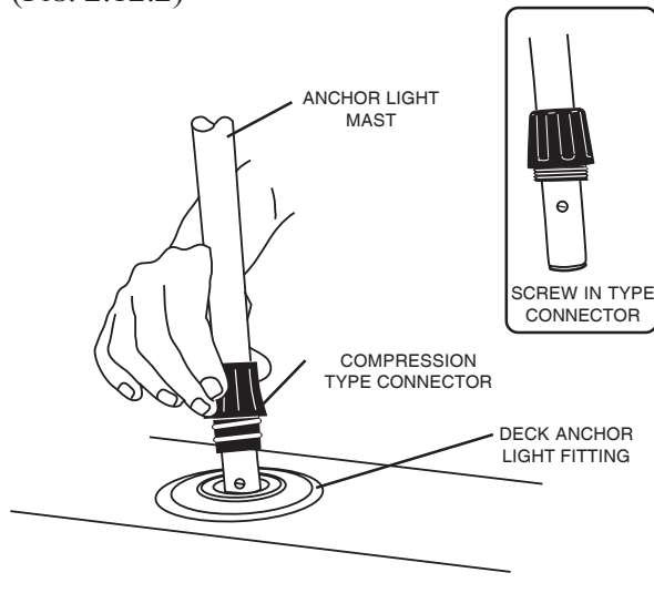
INSERTING THE REMOVABLE STERN ANCHOR LIGHT (FIG. 2.12.2)
