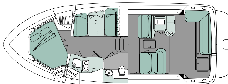
Cabin/Cockpit Layout
