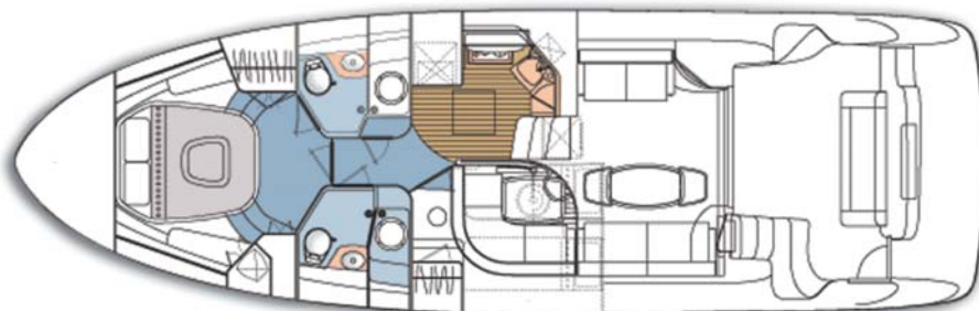
Cockpit/Cabin Layout
